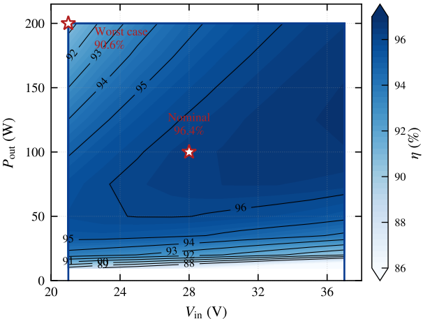
DCX200 R3, V_{\text{out}} = V_{\text{in}}/3
